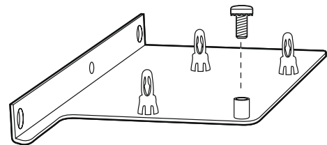
X-Mount M PN 53914 Used for mounting any Expander Board in a metal enclosure. Bracket attaches to heater mounting straps
